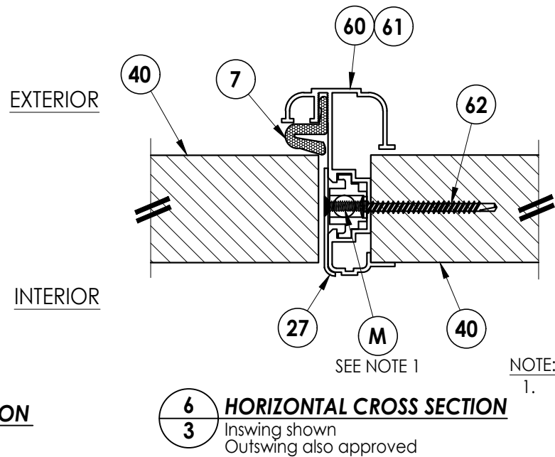
4 3 VERTICAL CROSS SECTION ADA Threshold
