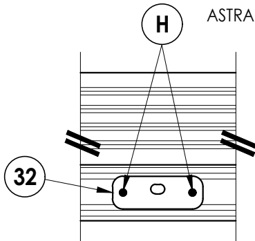
DETAIL 2 ASTRAGAL STRIKE PLATE @ SILL INSWING
